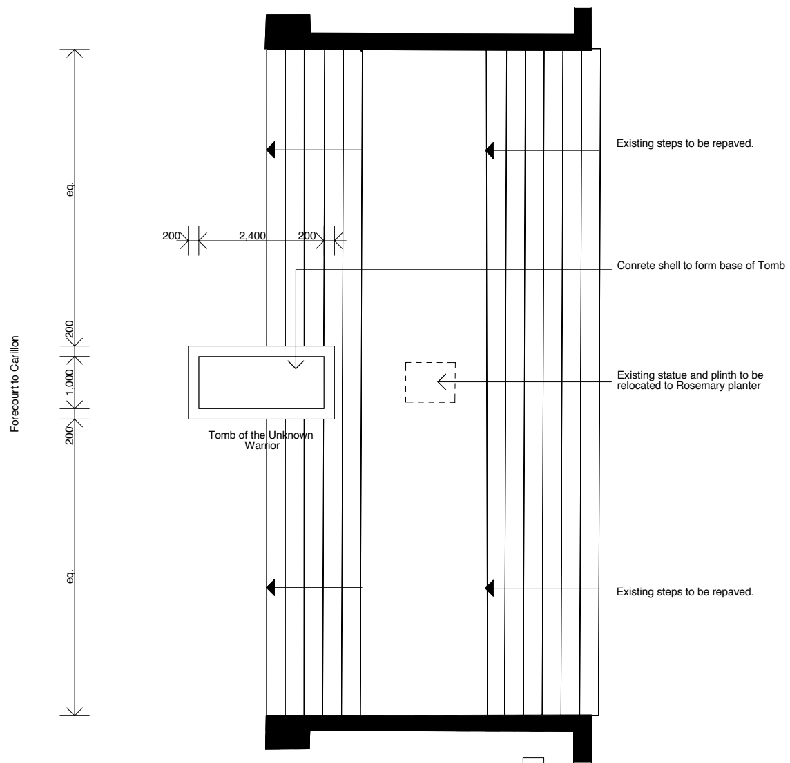
Plan of Tomb 1:100
